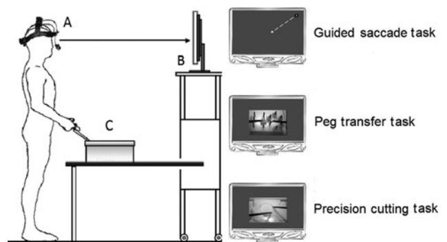
FIGURE 1. Experimental setup. Participants used the FLS box simulator for the laparoscopic tasks. The position of the simulator box was fixed (C). A USB Web camera (iREZ K2r USB; GlobalMedia Group, LLC; 640 \times 480 pixel resolution) fixed to the inside of the FLS box displayed the laparoscopic task area on the center of a computer monitor ( 28.2 degrees \times 21.1 degrees display area) facing the subject. The operating table's height was fixed at 87 cm, but participants could stand on a variable step if necessary. The monitor was mounted on a video cart and positioned about 170 cm above the floor level and about 57 cm from the participants' eyes. The EyeLink II helmet-mounted eye tracker (A) measured the subjects' eye movements. Adapted with permission from Rogers et al. 24
